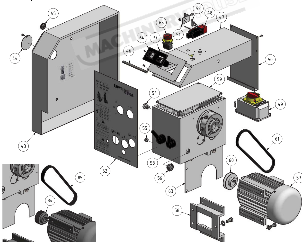
Abb.6-5: Spindelstock - Headstock
